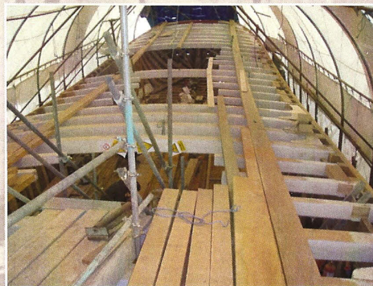
Same view - October 2009 - First deck planks being laid
